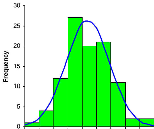
Figure 9. Example Histogram
